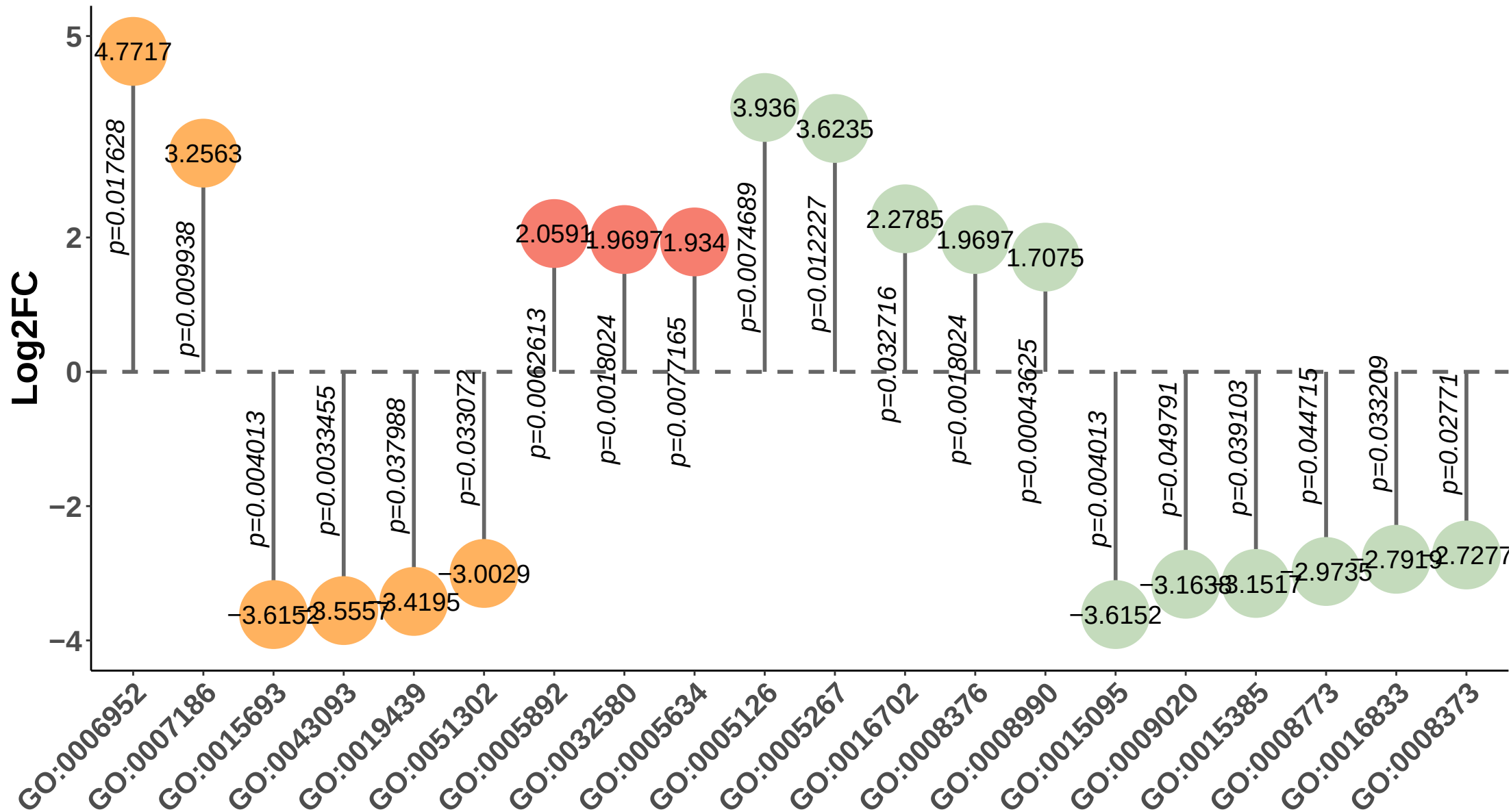
GO plot
